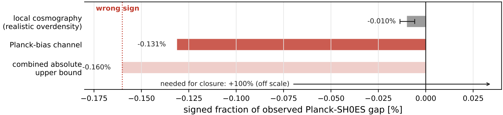
Figure V2.14.5. The Planck-SH0ES H_0 gap is about 8.4 percent; the current GCT biogenic-driving action shifts the inference in the opposite direction and supplies at most about 0.16 percent of the observed tension.
